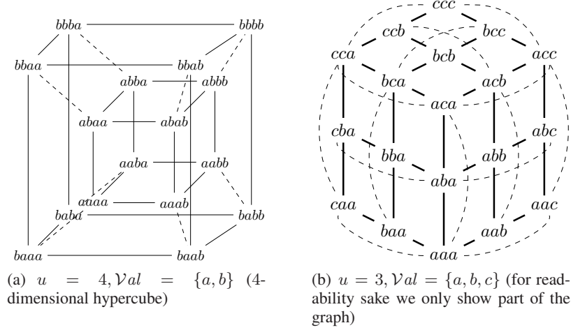
Fig. 7. Two (\text{Val}^u, \sim) graphs
