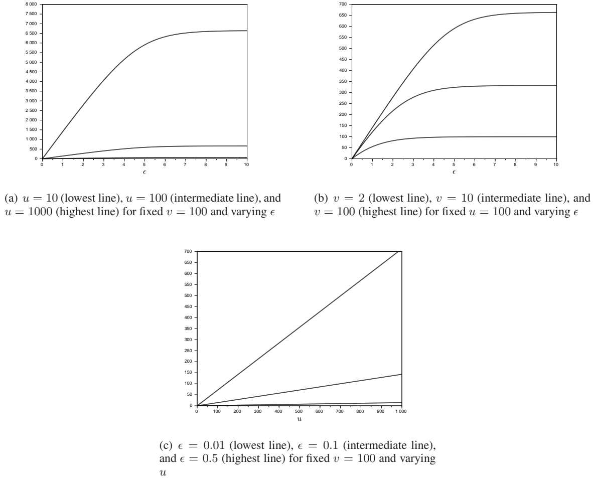
Fig. 8. Graphs of Bnd(u, v, \epsilon) for different configurations of u, v, \epsilon
