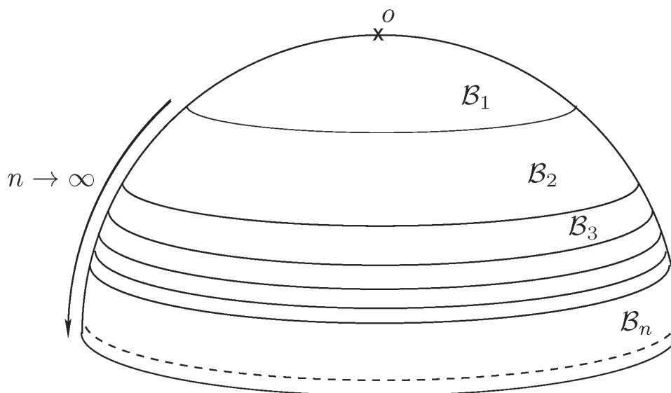
FIGURE 5.2: The open hemisphere is a CSLCG manifold.
