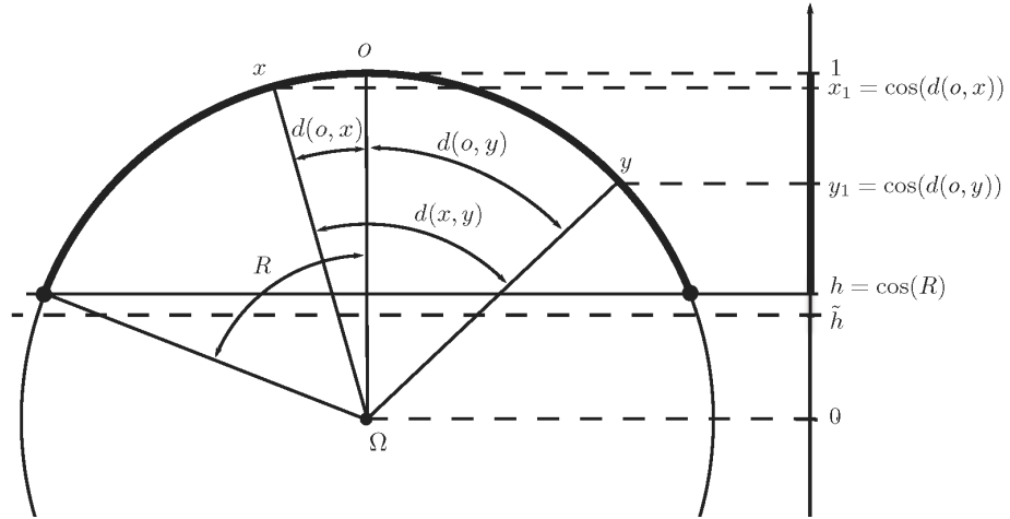
FIGURE 5.1: Bounded convex geometry for a regular geodesic ball of \mathcal{S}^1
