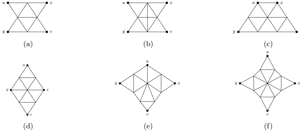
Figure 1: The six forbidden isometric subgraphs.
