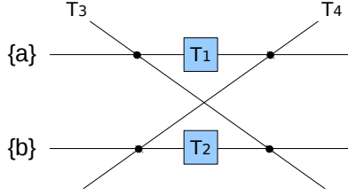
Figure 1: Non-monotonic Snapshots
