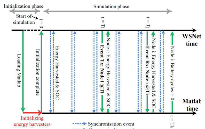
Fig. 3 Interactive co-simulation of WSNnet and Matlab
