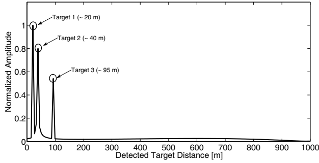
Figure 15. Range profile of multiple target for the case of FMCW radar.
