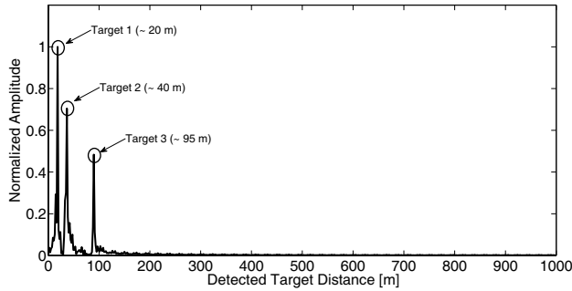
Figure 16. Range profile of multiple target for the case of OFDM radar.
