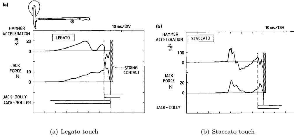
Figure 3: “Registration of acceleration at the hammer head and compression force in the jack ( mezzo forte , C_4 ). The force was measured by means of a piezofoil in the jack. The position of the accelerometer is marked with a triangle. Also shown are the contacts signals jack dolly and jack roller. (a) Legato touch and (b) Staccato touch.” Figure taken from [3].
