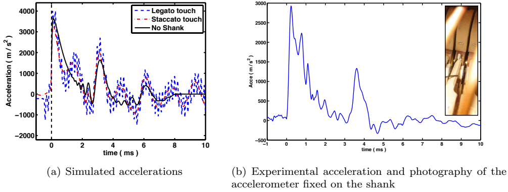
Figure 6: Comparison between simulated (left) and experimental (right) acceleration of the hammer head. The time scale has been shifted so that time 0 corresponds to the contact instant between the hammer head and the string.
