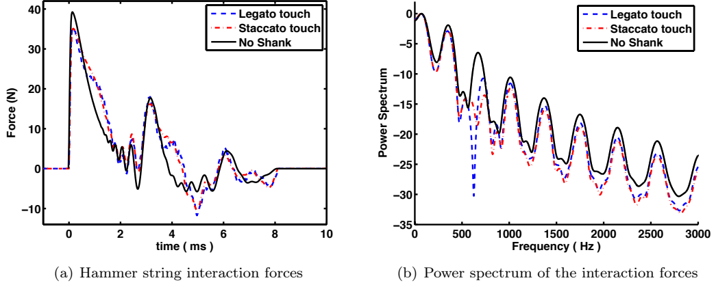
Figure 7: Temporal and spectral profiles of hammer head - string interaction forces obtained with different pianistic touches. The time scale has been shifted so that time 0 corresponds to the contact instant between the hammer head and the string.
