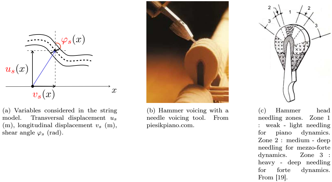
Figure 11: String model variables and theory of hammer voicing.
