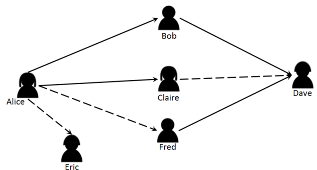
Fig. 1. Trust network
