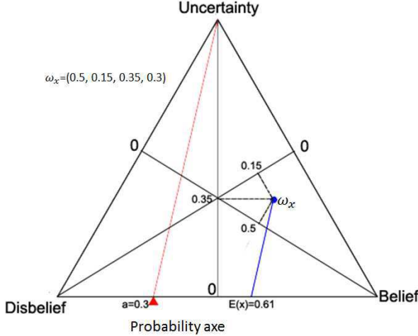
Fig. 2. Opinion
