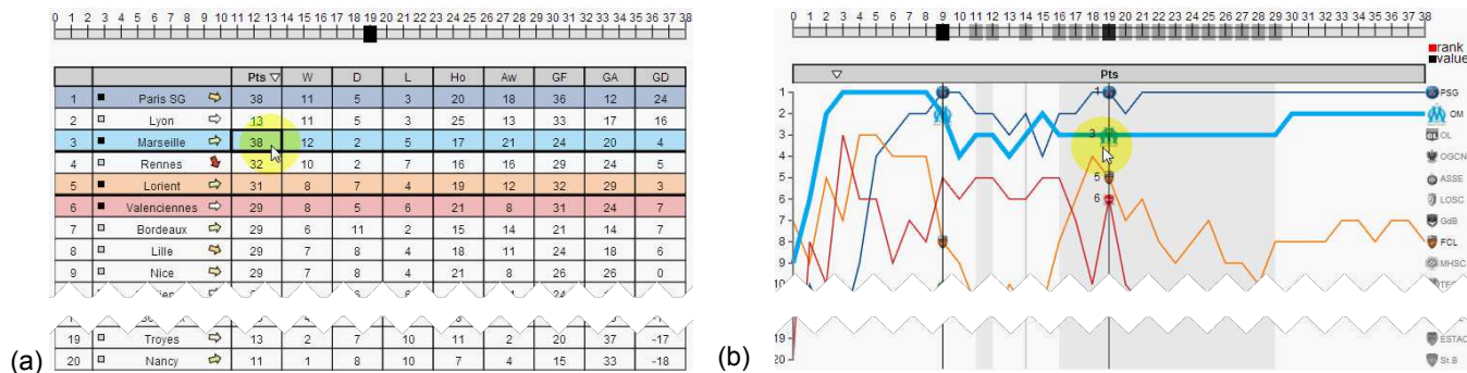
Figure 1. (a) DRAG-CELL and (b) VIZ-RANK, two novel temporal navigation techniques for ranking tables. DRAG-CELL is a direct manipulation technique to browse values over time by dragging them; VIZ-RANK uses transient visualization (line chart) to show the values of cells over time. For both techniques, the temporal slider on the top provides feedback on the current temporal navigation.
