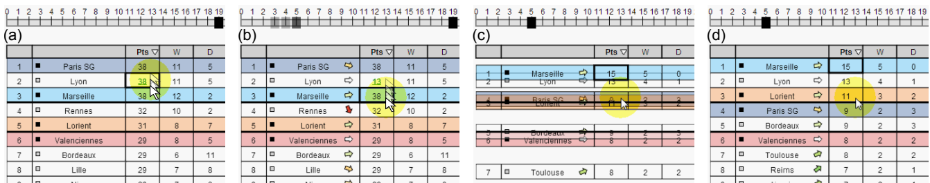
Figure 5. DRAG-CELL: (a) dragging up and down the value of a cell (in this case, Points of Team Lyon) makes this value change (b) for the set of values it can have, and colored arrows indicate how teams would behave if the drag was released (green to red arrows). (c-d) Releasing the drag animates the rows to their new position.
