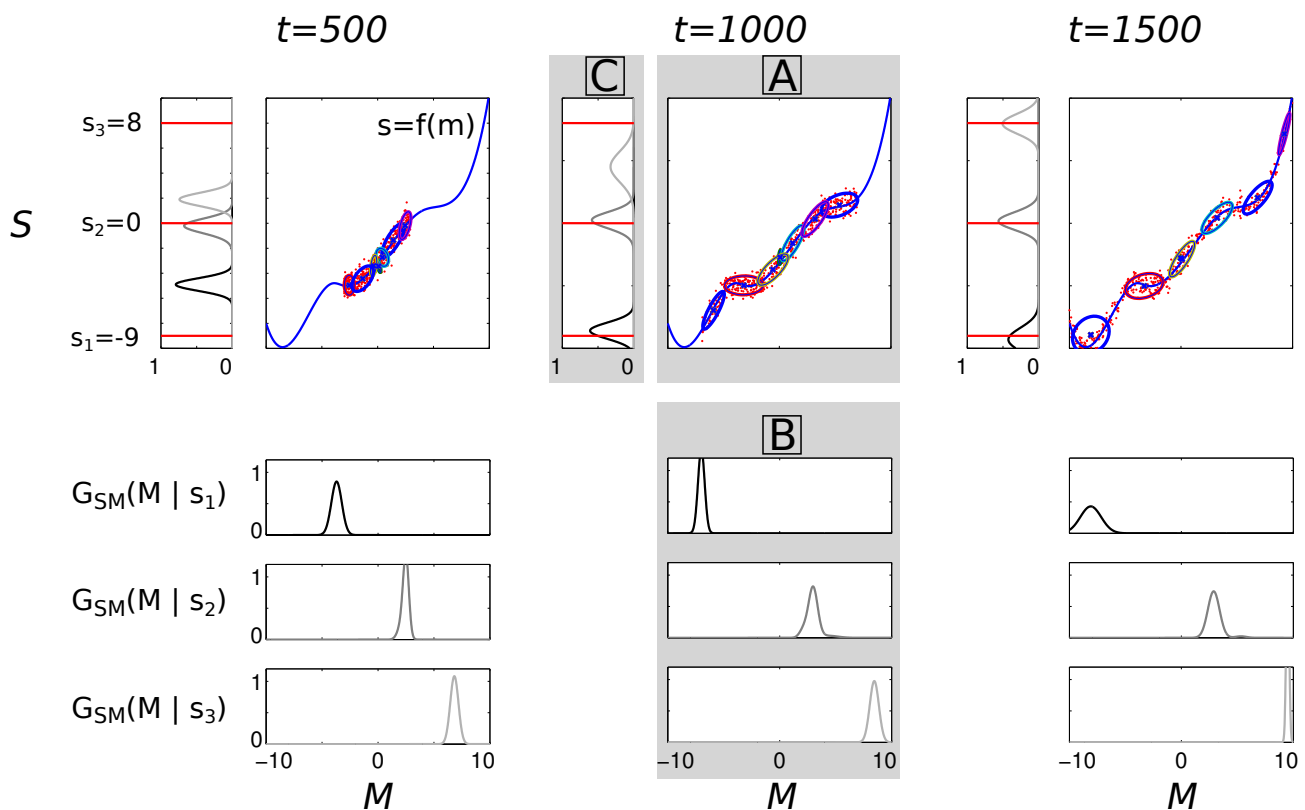
Figure 5. Illustration of incremental learning and inference in the sensorimotor model in a toy 2-dimensional sensorimotor space. The figure has three columns, corresponding to the state of a learning agent after 500, 1000 and 1500 sensorimotor experiments ( t = 500, 1000, 1500 ). Each column is divided in three panels A, B and C, as indicated in the middle column (boxed letters in gray panels). X-axis ( M space) and y-axis ( S space) of A are shared by B and C, respectively. A) The unknown function s = f(m) is represented by the blue curve. The red points are the sensorimotor experiments made at this stage (i.e. until the corresponding time index t ): when m is produced, s = f(m) + \epsilon is perceived, where \epsilon is here a Gaussian noise with a standard deviation of 0.5. The ellipses represent the state of G_{SM} learned from the sensorimotor experiments, which is here a GMM with 6 components (each ellipse represents a 2D Gaussian). B) The three vertically-aligned plots show the motor distributions G_{SM}(M | s_g) for 3 different goals, s_1 = -9.0 (top), s_2 = 0.0 (middle), and s_3 = 8.0 (bottom), in each of three columns (i.e. at the three time indexes). They are inferred from G_{SM} in A using Bayesian inference. C) The probability distributions on S (rotated 90 degrees anti-clockwise) resulting from sampling motor configurations according to G_{SM}(M | s_g) , to reach the three goals s_1 , s_2 , and s_3 , the shade of grey of each one corresponding to that used in B: this means for example that, at a given time index t , producing motor commands according to the distribution G_{SM}(M | s_3) (panel B, bottom) will result in sensory consequences following the darker distribution in panel C. The three considered goals s_1 , s_2 and s_3 are represented by the three horizontal red lines, which are the same in the three columns. The distributions in C thus reflect how the learner is able to reach one of the three considered goals using the current state of its sensorimotor model: we observe that at t = 500 , it can only reach s_2 = 0 ; at t = 1000 , it can also reach s_1 = -9 and at t = 1500 it can reach those three goals.
