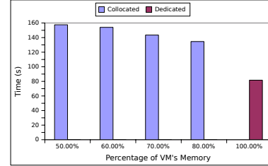
Figure 9. The execution time of the Kabsch-based application on a fixed set of input data. The percentage of the VM memory used by the application is increased, when using the collocated storage. The final bar represents the application execution time using all VM memory when the storage is moved to dedicated nodes
