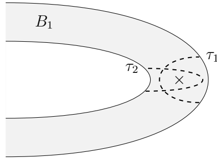
Figure 19: Two incompatible pictures in the universal cover ( \tilde{B}_1 is in grey)
