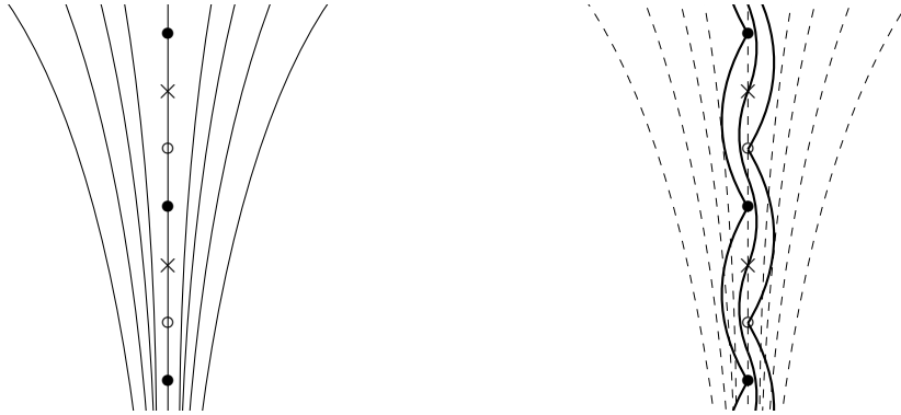
Figure 7: Constructing proper homotopy streamlines in the bad case
