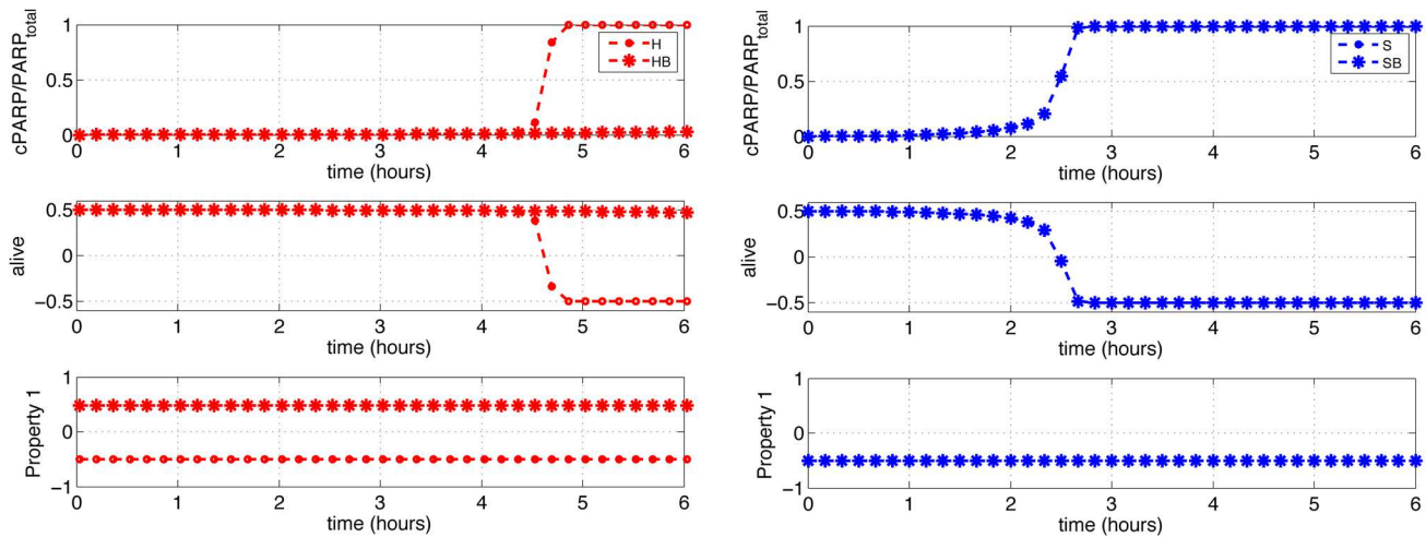
Figure 9. Evaluation of STL properties. Temporal evolution of the ratio cPARP/PARP_{total} , of the value of the property alive := cPARP/PARP_{total} < 0.5 , and of Property\ 1 := always_{[0-6h]}(cPARP/PARP_{total} < 0.5) for HCT116 and OE-Bcl2 HCT116 cells (left), and SKW6.4 and OE-Bcl2 SKW6.4 cells (right). When the concentration of cleaved PARP increases, the value of the alive property gradually decreases from a positive value (“true”) to a negative value (“false”). Property\ 1 at time t evaluates to the minimal value of alive at all future times. So, Property\ 1 simply captures whether at all times alive holds. doi:10.1371/journal.pcbi.1003056.g009
