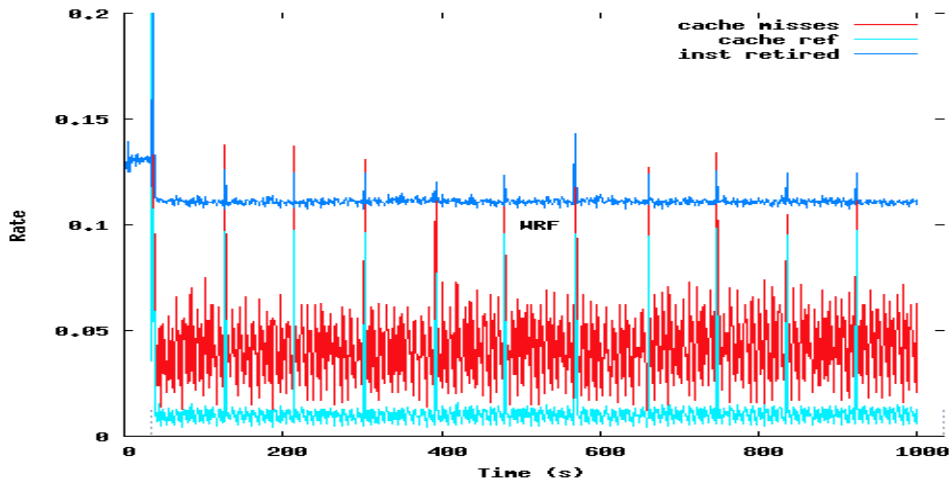
Figure 2: Phase changes detection using the similarity between consecutive execution vector as similarity metric.
