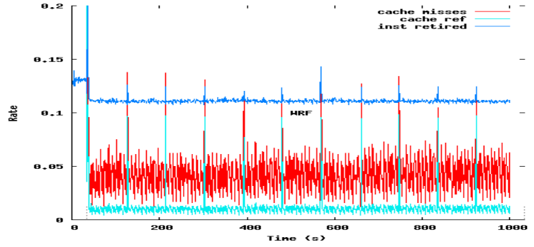
(b) Cache reference and miss rates along with retired instructions rate.
