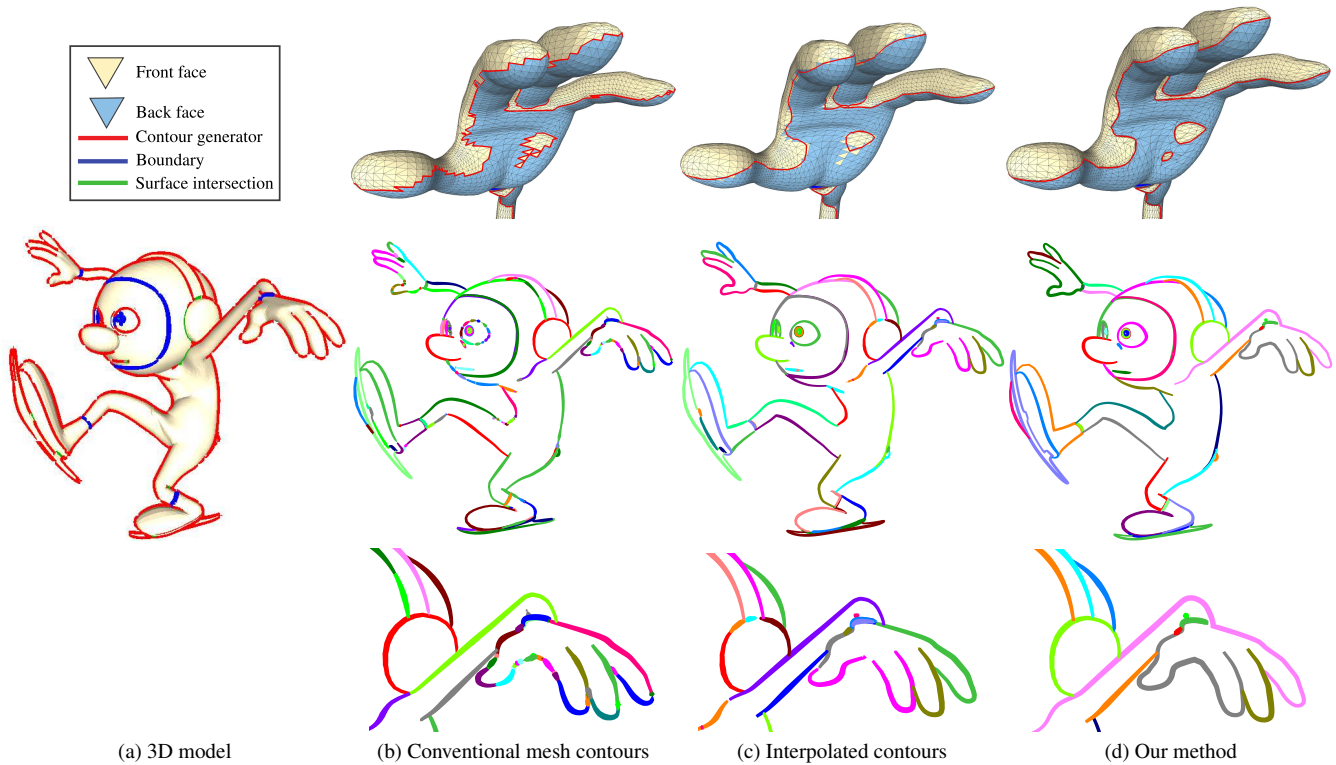
Fig. 1. Contour extraction from a smooth 3D surface. (a) The object is modeled as a collection of Catmull-Clark surfaces. We extract contours (red), boundaries (blue), and surface-intersection curves (green). (b) Contours of a conventional surface tessellation exhibit overly-complex topology. (c) Smooth interpolated contours [Hertzmann and Zorin 2000] have simpler topology. However, because they are not true contours of the tessellation, there are visibility errors, such as the gap in the left hand, and broken outline curves. (d) Our method generates a mesh tessellation such that the mesh contours have accurate topology for the underlying surface. Colors: Front-faces are drawn in yellow, and back-faces in blue. All strokes are rendered with tapering and random colors, in order to visualize the extracted topology. Red © Pixar
