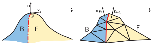
Fig. 3. Contours. The contour generator is the boundary between the front-facing and back-facing parts of a surface, as seen from a camera center \hat{c} . Left: For a smooth surface, these points have a surface normal \mathbf{n} perpendicular to the view vector \mathbf{v} = \hat{c} - \mathbf{p} . Right: For a triangle mesh, the contour generator comprises the mesh edges between front-faces and back-faces.
