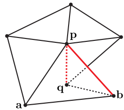
Fig. 20. A curtain-fold cusp in the contour. Edge \overline{\mathbf{pb}} is an exterior contour. Edge \overline{\mathbf{pq}} is an interior contour, indicating that it is occluded by a nearby face. Vertex \mathbf{p} is thus a curtain-Fold cusp [Markosian et al. 1997]. (A cusp of the mesh boundary curve occurs in the same configuration, but with triangle \mathbf{pqb} removed.)
