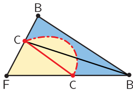
Fig. 19. Missing zero-crossing on a CB edge. A zero-crossing is missed by our algorithm; the CBB and CCB triangles are not Strongly Contour-Consistent. Yet, the mesh contour (CC edge) is still topologically equivalent to the smooth contour segment (dashed curve).
