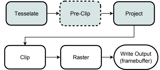
Figure 2: Rendering pipeline proposed for wide FoV real-time rendering. Gray stages are implemented in shaders. The new pre-clip stage (dashed) represents our main contribution.
