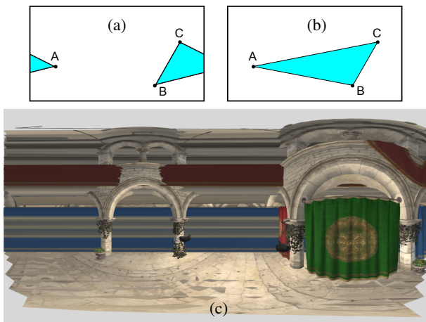
Figure 4: Rasterization issue for triangle projected across the discontinuity of an equirectangular projection. (a): desired rendering in the final viewport. (b): the surface actually generated. (c): the problem on a real scene: here, the triangles composing the red and blue drapes on the very right are rasterized across the whole viewport.
