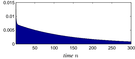
Figure 2. Distribution of the time to reach state P. The mean time is 134 years and the standard deviation is 130 years, this standard deviation is rather high as the time to reach P is exponentially distributed.
