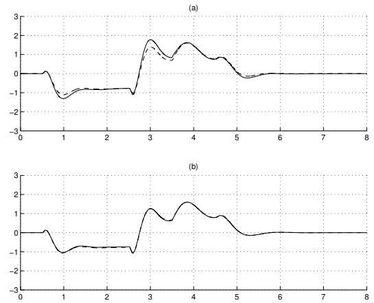
Fig. 5. Real parameters. v_y (solid) and v_{y,ref} (dashed) [m/s vs s]: a) PI-based controller; b) ST-based controller.
