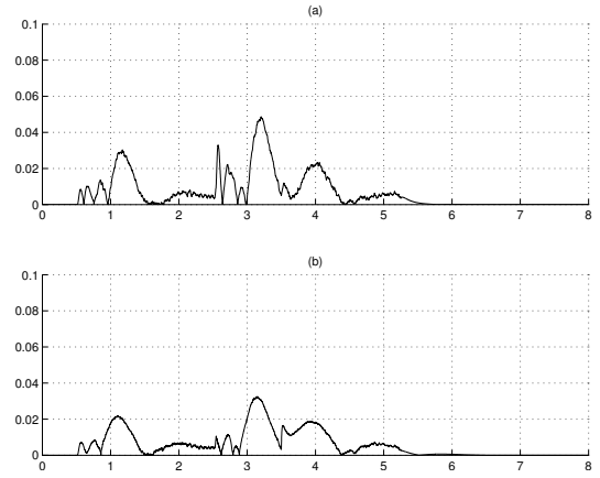
Fig. 4. Nominal parameters. Absolute tracking error |\omega_z - \omega_{z,ref}| [rad/s vs s]: a) PI-based controller; b) ST-based controller.
