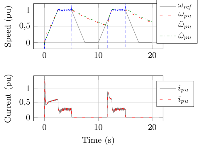
Fig. 5. Sensorless speed control performance at zero current in the presence of estimator
