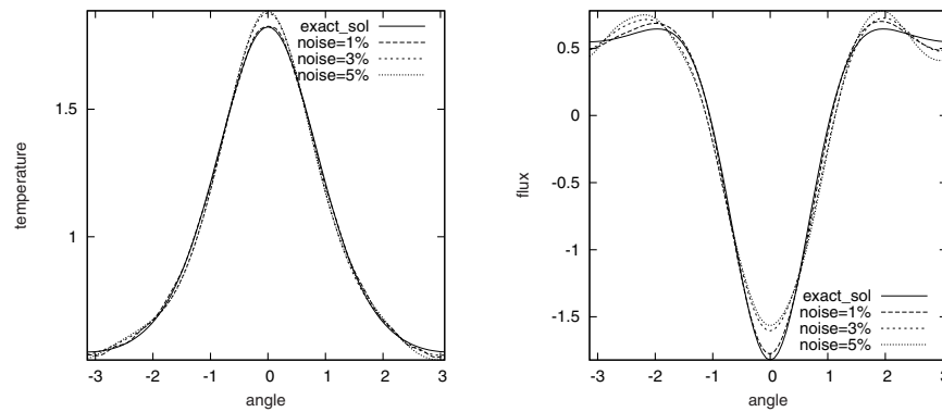
FIG. 5.1. Test case A. Reconstructed smooth Dirichlet ( \tau_N , left) and Neumann ( \eta_N , right) data over \Gamma_i . The profiles are presented at convergence and for various noise levels \sigma \in \{1\%, 3\%, 5\%\} . The corresponding traces of the exact solution are also plotted. The finite element computations are performed with 1529 nodes and 2788 triangles.
