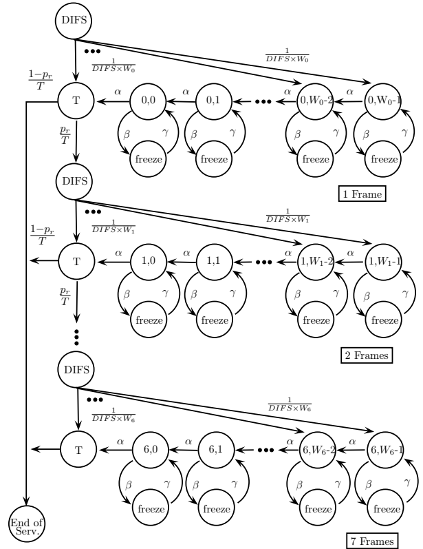
Figure 4: Local CTMC model for each node.
