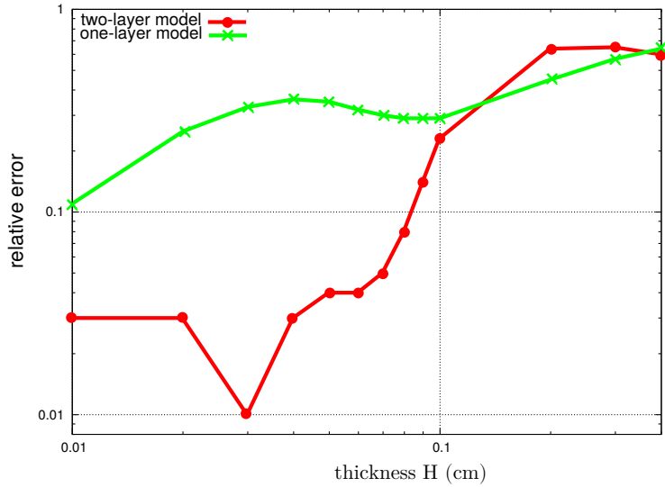
Figure 2: Convergence graph. Green : 1x2D model. Red : 2x2D model
