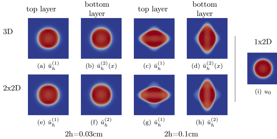
Figure 1: Comparison of the depolarisation maps of the 3D (fig. 1(a) to 1(d)), 2x2D (fig. 1(e) to 1(h)) and 1x2D (fig. 1(i)) cases, at t = 9ms . N.B.: as the 1x2D model does not depend on h , only one snapshot is displayed.
