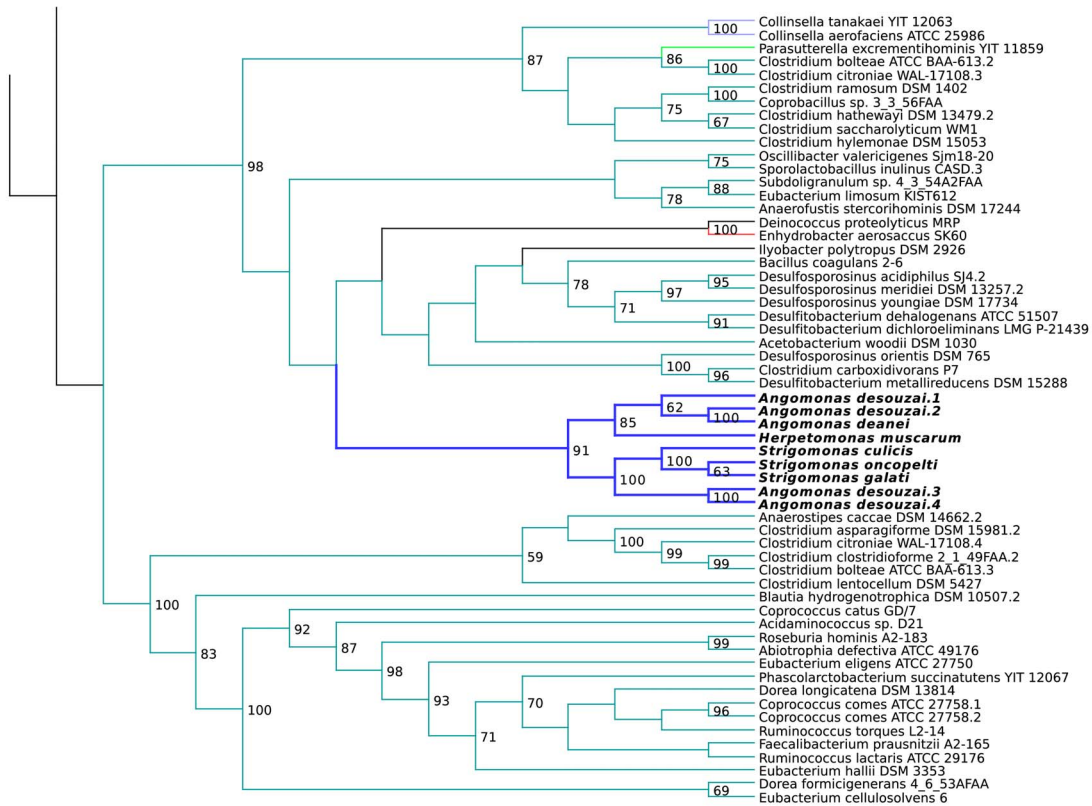
Figure 9. Maximum likelihood phylogenetic tree of ketopantoate reductase (EC:1.1.1.169). A - overall tree, colored according to taxonomic affiliation of each taxon, as per the legend on the left; distance bar only applies to panel A. B - details of the region of the tree where the Trypanosomatidae are placed. Values on nodes represent bootstrap support (only 50 or greater shown). Panel B is meant to only represent the branching patterns and do not portray estimated distances between sequences. doi:10.1371/journal.pone.0079786.g009
