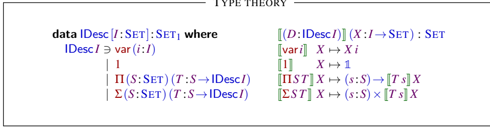
Fig. 2: Universe of inductive families
