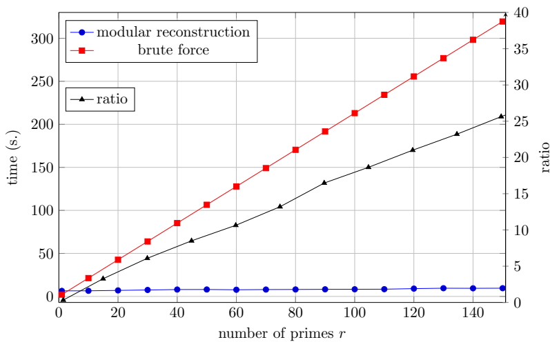
FIGURE 3. Timings for the modular reconstruction algorithm and brute force.
