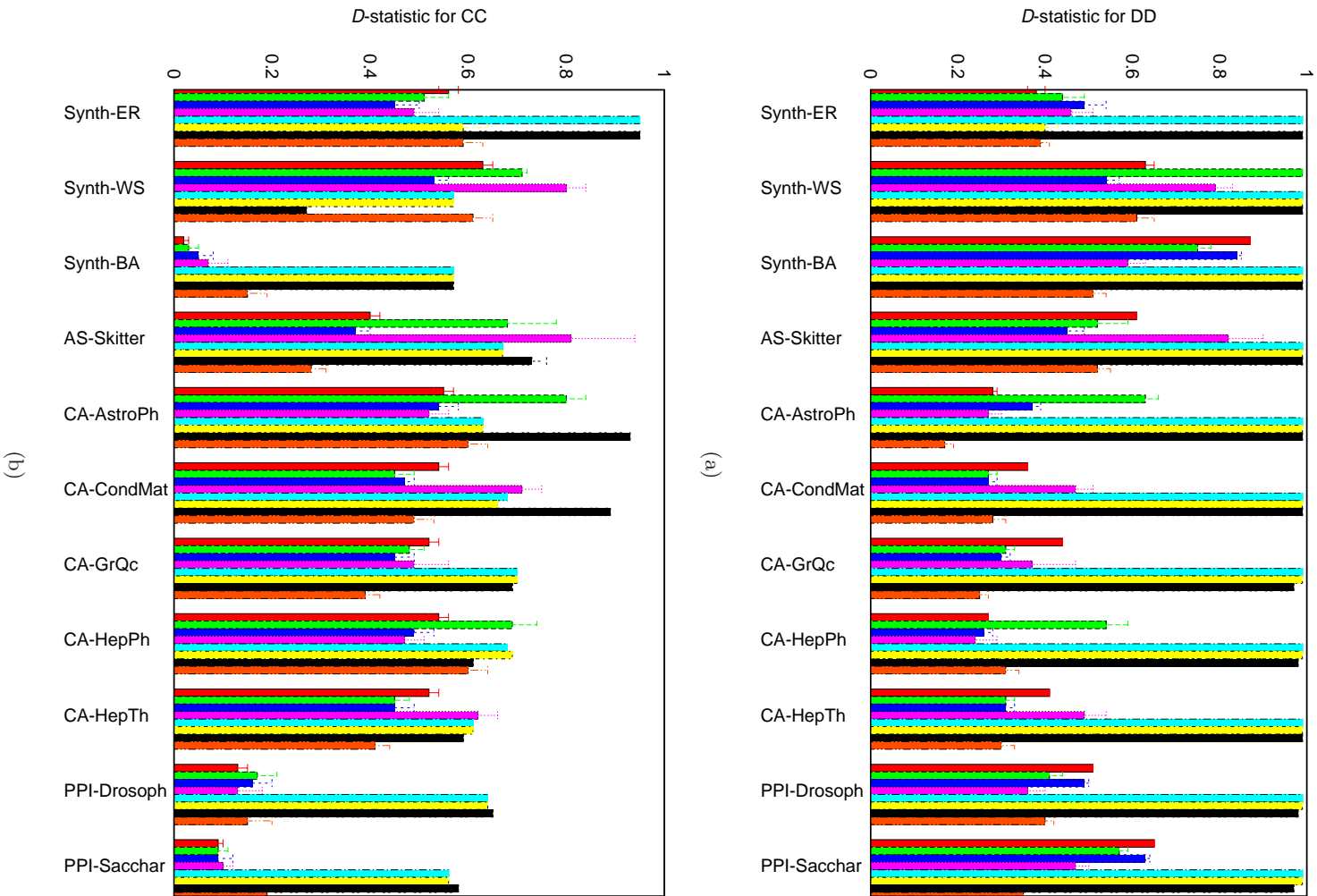
Figure 8: Average D -statistic values for degree distribution and clustering coefficient on the networks listed in Table 1.
