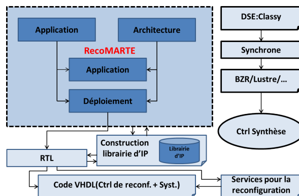
FIGURE 1 – Flot FAMOUS
