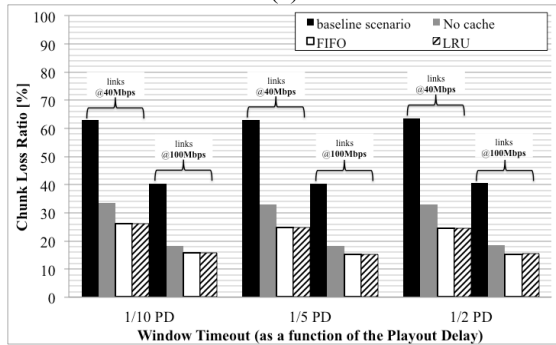
Figure 1. Chunk Loss Ratio when the playout delay has been set to (a) 10s and (b) 20s.
