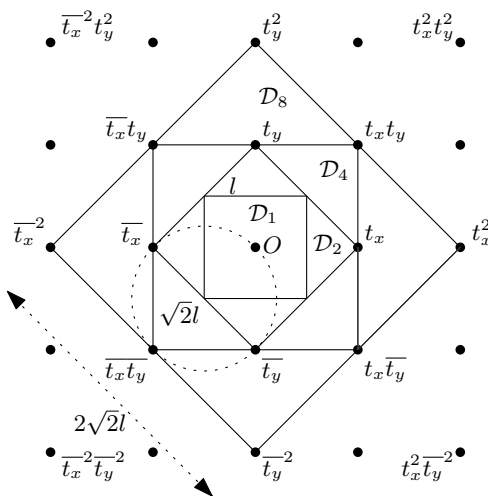
Figure 11: Euclidean case.
