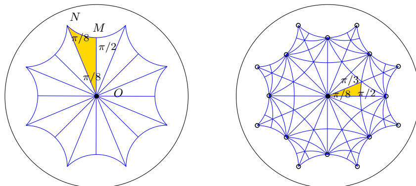
Figure 5: Partition of a fundamental domain for \mathcal{G} into fundamental domains for the triangle groups T(2, 8, 8) (left) and T(2, 3, 8) (right), where small circles show the elements of the orbit T(2, 3, 8)O in the octagon.
