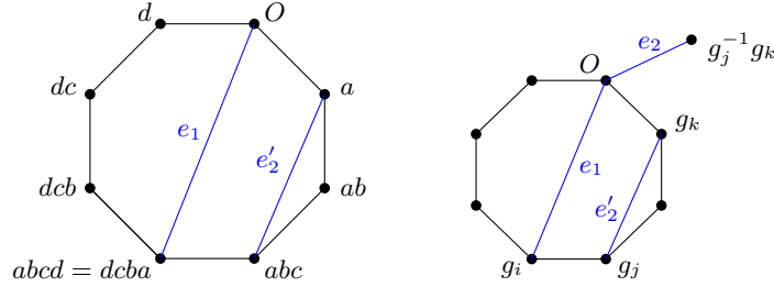
Figure 18: Enumerating edges.
