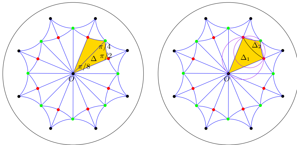
Figure 19: (left) Partition of \mathcal{D}_O(\mathcal{G}) into fundamental domains for T(2, 4, 8) . (right) Triangles \Delta_1, \Delta_2 obtained by edge-flipping.
