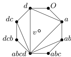
Figure 12: Proof of Proposition 21: avoiding edge with vertices O and abcd .
