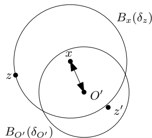
Figure 3: Proof of Proposition 3
