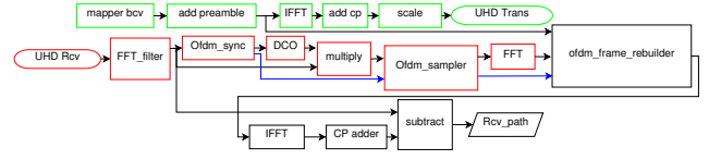
Fig. 2. Flow chart of ofdm_full_duplex
