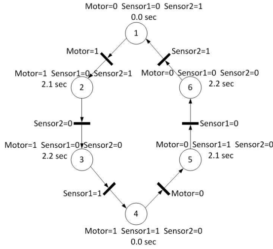
Figure 5.6: Baseline SDS inferred model
