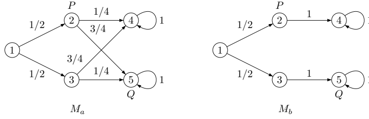
Fig. 4. Markov chains distinguishable by PCTL^* formulas
