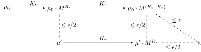
Fig. 9. Proof sketch of Lemma 8.5
