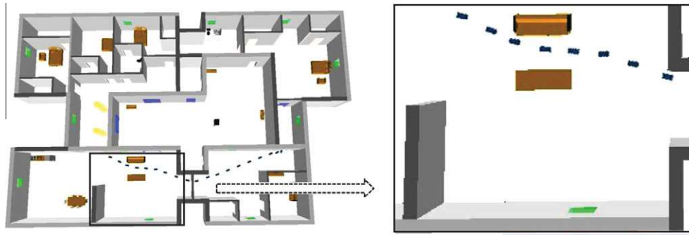
Fig. 14. An example shows the disadvantage of the traditional FMM in path planning. For the narrow opening between the desk and the sofa, the path generated by the traditional FMM directly goes through it. In practice, the narrow opening is too narrow so that it is difficult to pass for people.
