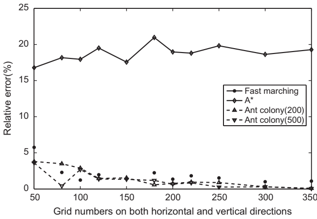
Fig. 9. Illustrating the relative errors of FMM, A* algorithm and the ant colony algorithm on different grid resolutions, where the ant colony algorithm is respectively tested with 200 iterations and 500 iterations.
