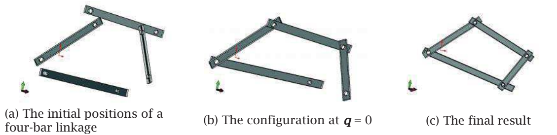
Fig. 5: The solving process of a four-bar linkage
