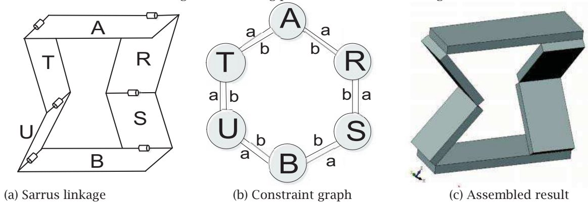
Fig. 6: A Sarrus linkage and its constraint graph
