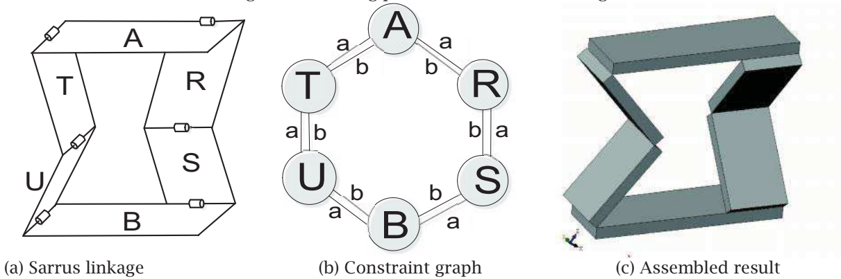
Fig. 6: A Sarrus linkage and its constraint graph
