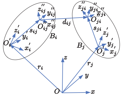
Fig. 3: The representation of relative motions of two bodies
