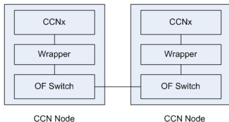
Figure 1: Integration of the Wrapper in nodes
