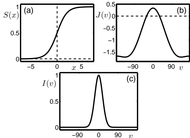
Fig. 1 Model features and stimulus. (a): The smooth (infinitely differentiable) sigmoidal firing rate function S(x) . (b): The convolutional kernel J is a three-mode approximation of a Mexican hat connectivity. (c): The simple stimulus is a Gaussian bump centered at v = 0^\circ .
