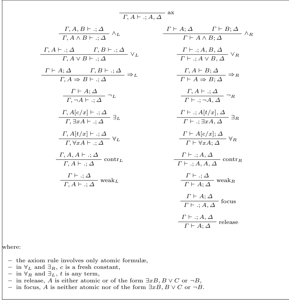
Fig. 3. Focused classical sequent calculus
