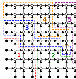
Fig. 6: Convex-partition of the CDAG for the code in Fig. 2 for N = 10 .
