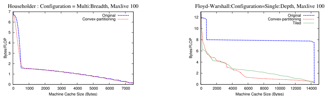
Fig. 4: Reuse distance analysis for Householder and Floyd-Warshall
