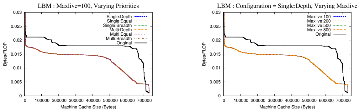
Fig. 16: Results with different heuristics for 470.lbm
