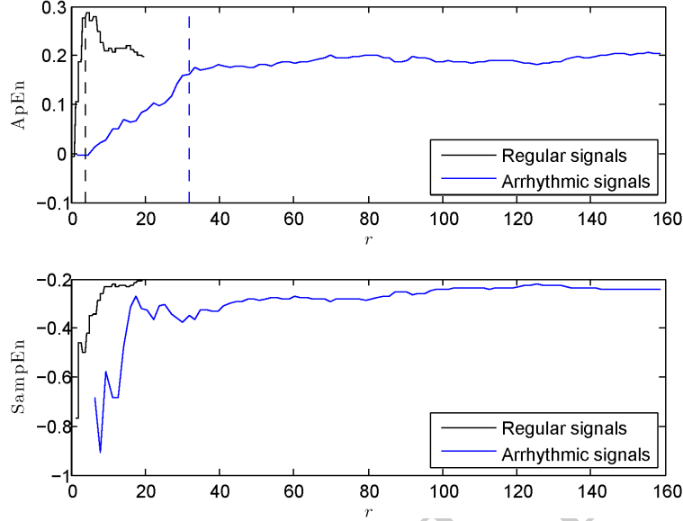
Figure 8. ApEn and SampEn for periods of EFP signals
