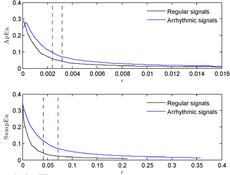
Figure 6. ApEn, SampEn for EFP signals. Dashed line indicates the conventional value of r = 0.2 \times \text{standard deviation of the signal}
