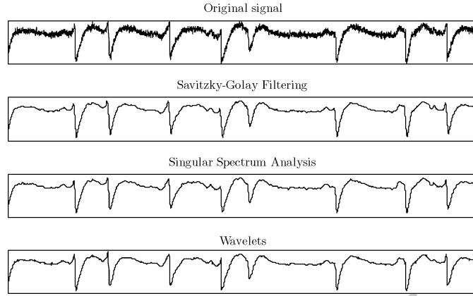
Figure 3. Comparison of three denoising methods, arrhythmic EFP signals
