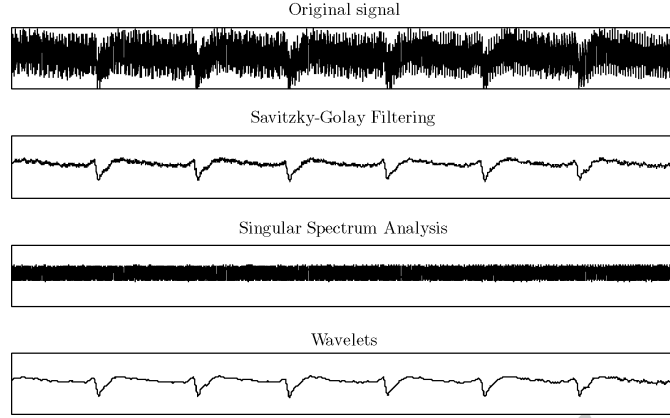
Figure 5. Comparison of three denoising methods, very noisy regular EFP signals
