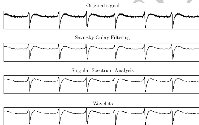
Figure 2. Comparison of three denoising methods, regular EFP signals
