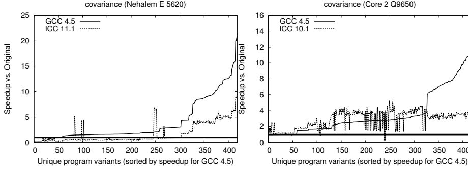
Fig. 1 Performance distribution for covariance
