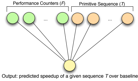
Fig. 6 Our speedup prediction model takes in two inputs. The first input is a characterization of the program consisting of a feature vector F of performance counters. The second input is a set of possible optimizations from the polyhedral optimization space. The target value for this predictor is the speedup of a specific optimization set T over baseline.
