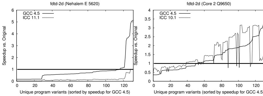
Fig. 2 Performance distribution for fdt-d-2d
