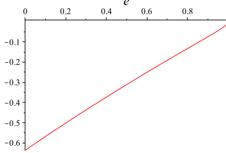
Fig. 4 Numerical plot of the function (73) on the interval [0, 1) . Obtained with Maple 15.
