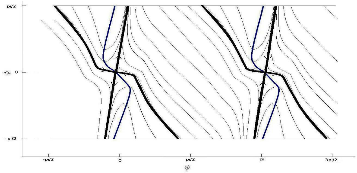
Fig. 1 Numerical plot (obtained using Matlab) of the stable and unstable manifolds (bold) and trajectories through a number of arbitrary initial values in C for the full control case. The other curve shown is \psi = Z_b(\varphi) .
