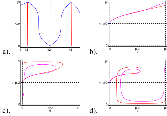
Fig. 4. a). Evolution of q_1^1 with respect to k , p_\theta = 10^{-4} . In red: \theta(t_*^1(p_\theta, k)) , in blue: \varphi(t_*^1(p_\theta, k)) , k_1 \approx 1.061 , k_2 \approx 1.250 , k_3 \approx 1.429 . Figures b)- d): the deformation of one branch ( p_\varphi = -2 and p_\theta \geq 0 ) of the conjugate locus w.r.t. the parameter k \in [1, k_3] : (b) k = 1.0, 1.05 ; (c) k = 1.1, 1.2 ; (d) k = 1.3, 1.4 .
