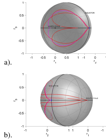
Fig. 7. Conjugate locus on the sphere, magenta curve: k = 1 (Grushin metric). a). red curves: k = 0.8, 1.15 ; b). red curves k = 1.2, 1.25 .
